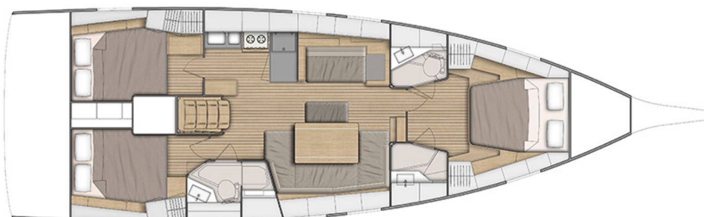
OPTION - 3 CABINS + 2 HEADS
