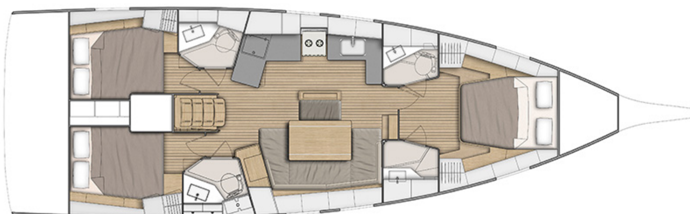
OPTION - 3 CABINS + 3 HEADS
