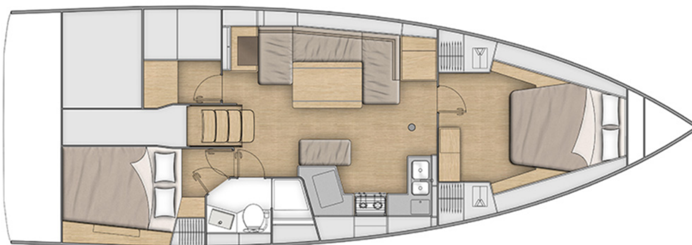
OPTION - 2 CABINS + 1 HEAD
